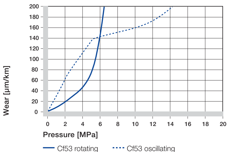
Graph 20.9: Wear for rotating and oscillating applications as a function of the pressure (Cf53 hardened and ground steel shaft)
